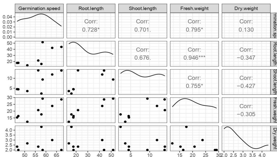
Figure 2. The correlation analysis among the studied traits in seed germination of L. iberica
