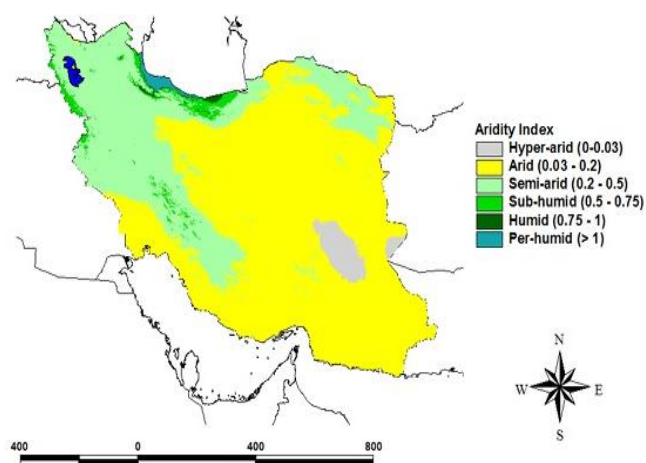
Figure 1. Aridity classes in Iran (Garshasbi, 2014).
