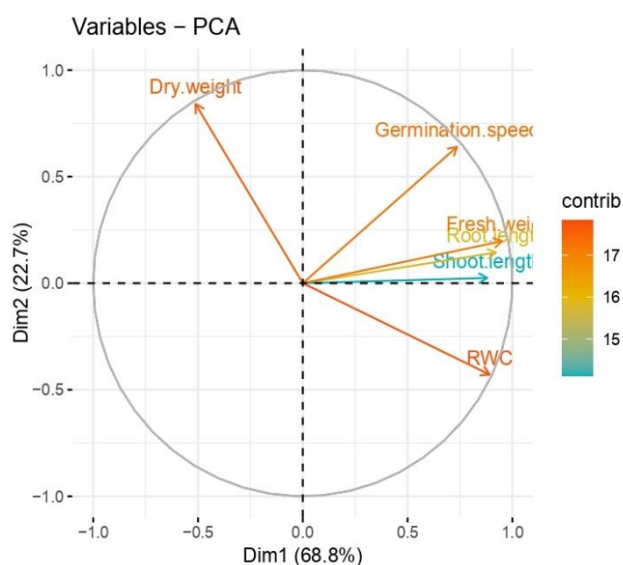
Figure 4. The bi-plot of PCA based on seed germination traits of L. iberica plant under drought stress.
