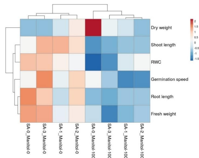
Figure 3. Heat-map cluster analysis of traits studied in seed germination of L. iberica
